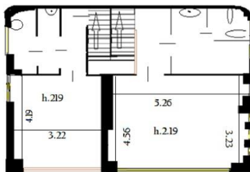
PIANO SOPPALCO
